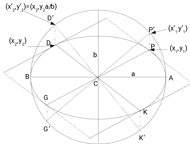
Figure 3b: Projecting the ellipse points P , D , G and K onto P'D' , G' and K' on the eccentric circle.
