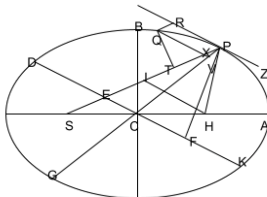
Figure 1: Based on Newton’s diagram for problem 3. A planet P moves in an elliptic orbit APQB about a center of force S located at a focus of the ellipse.
