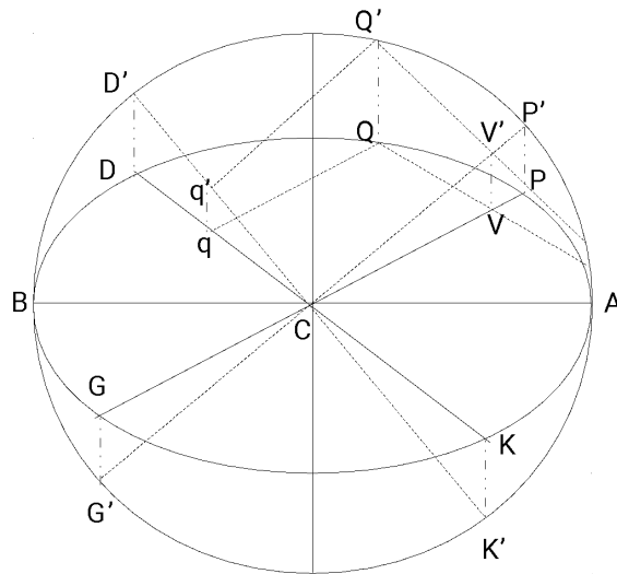
Figure 2b: projecting the ellipse points P, Q, D, G and K onto P', Q', D', G' and K' on the eccentric circle.
