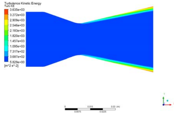
Figure 15: Contours of conventional nozzle Turbulence Eddy Dissipation
