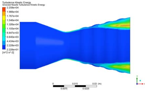
Figure 14: Contours of grooved nozzle Turbulence Kinetic Energy
