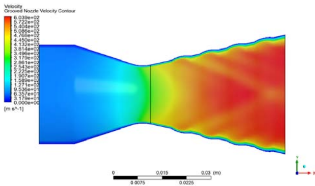
Figure 12: Grooved nozzle velocity contours
