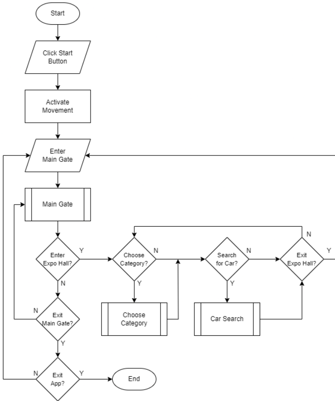
Figure 1: Main Application Flowchart
